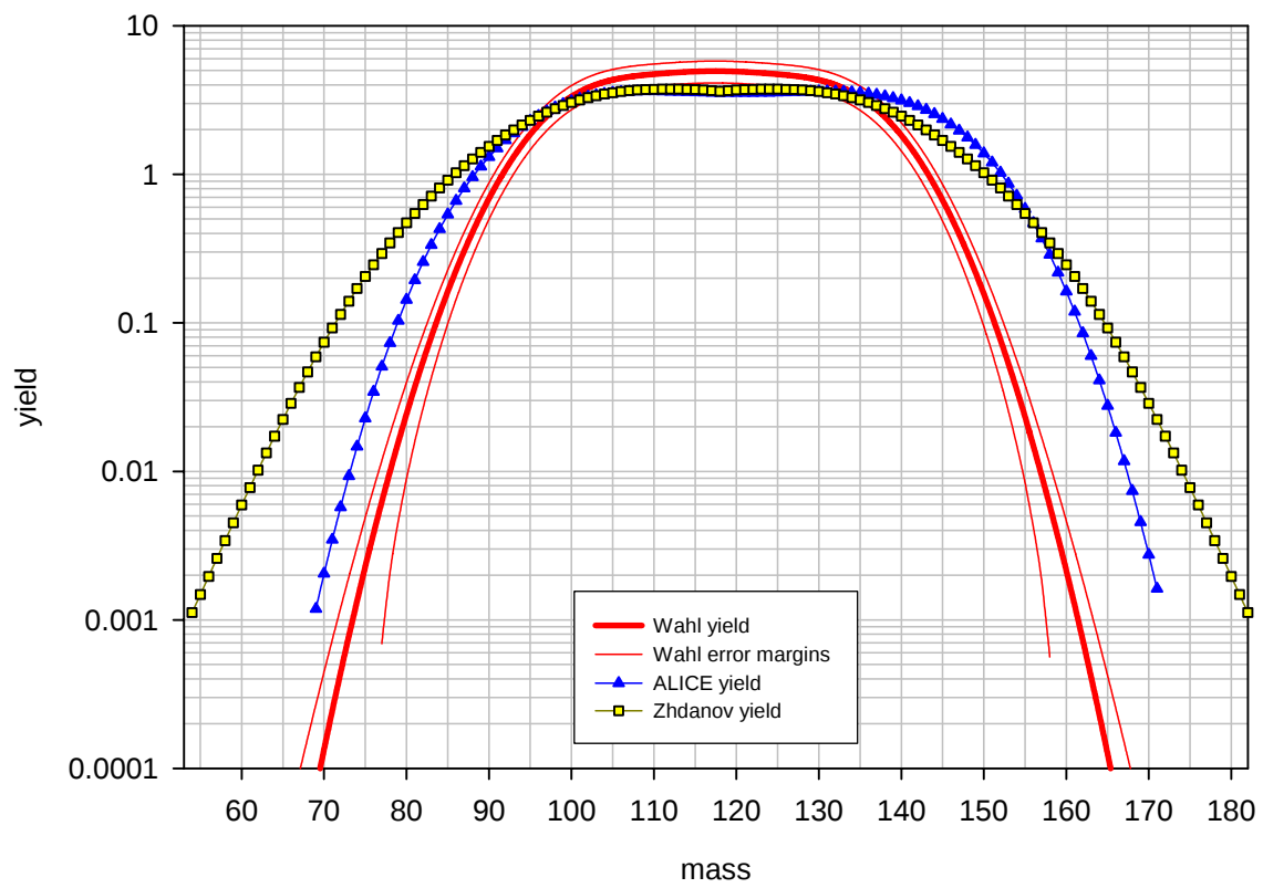
Benchmark B: ^{241}\text{Am} at 160 MeV, pre-neutron emission mass distribution
